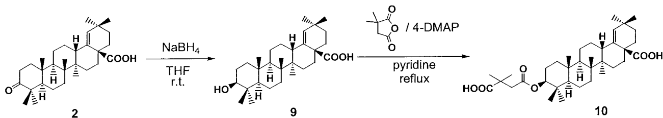
Scheme 1. Modification of Moronic Acid ( 2 )
