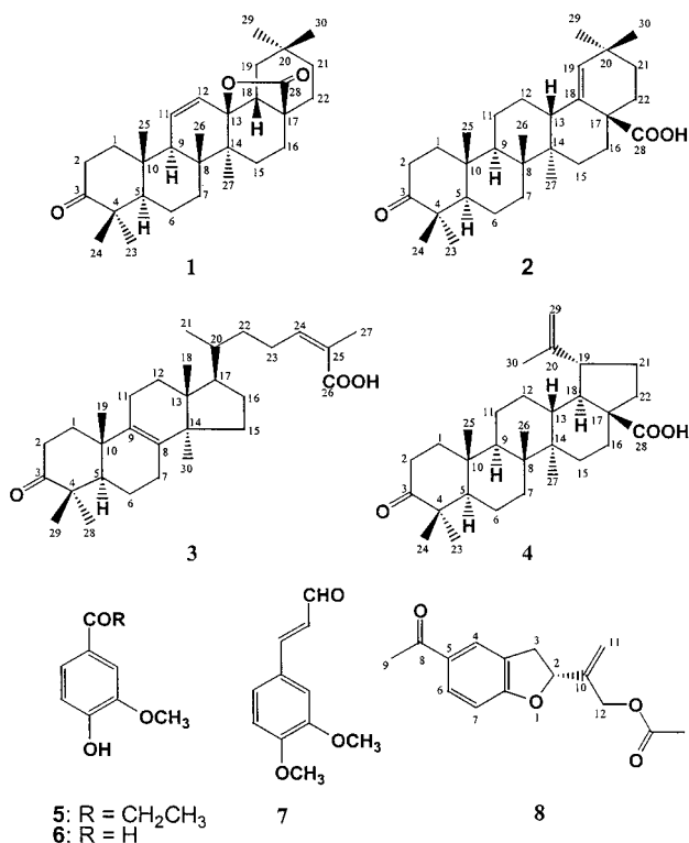
Figure 1. Compounds isolated from Brazilian propolis.
